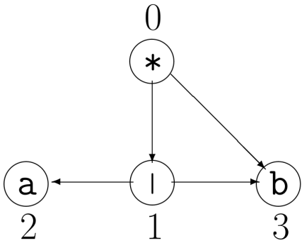
Figure 1: An AND-OR graph
