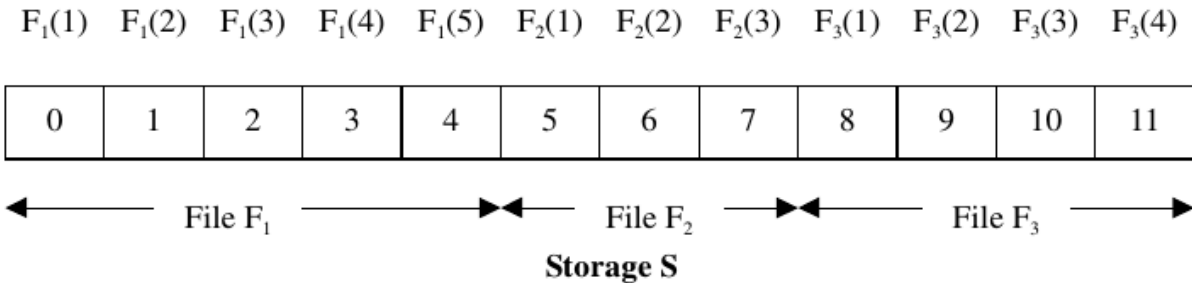
Fig. 1: An example of three files being stored in the storage S .
