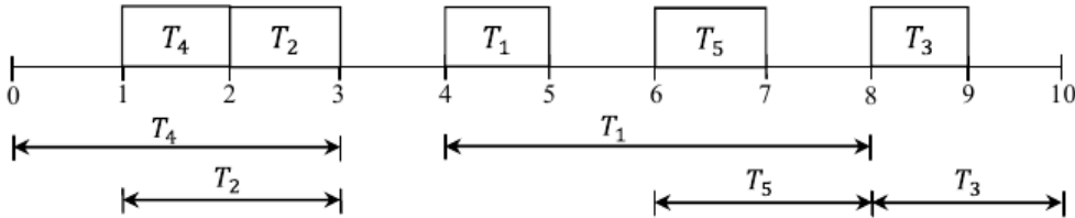
Figure 1. A schedule with 3 idle periods.
