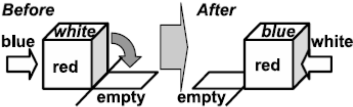
Figure 5: Rolling a cube
