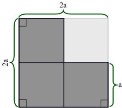
Figure 1: Defining L
