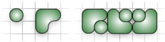
The precise sizes of the cakes Wolfgang makes and one way to pack them in a box of length 6.
